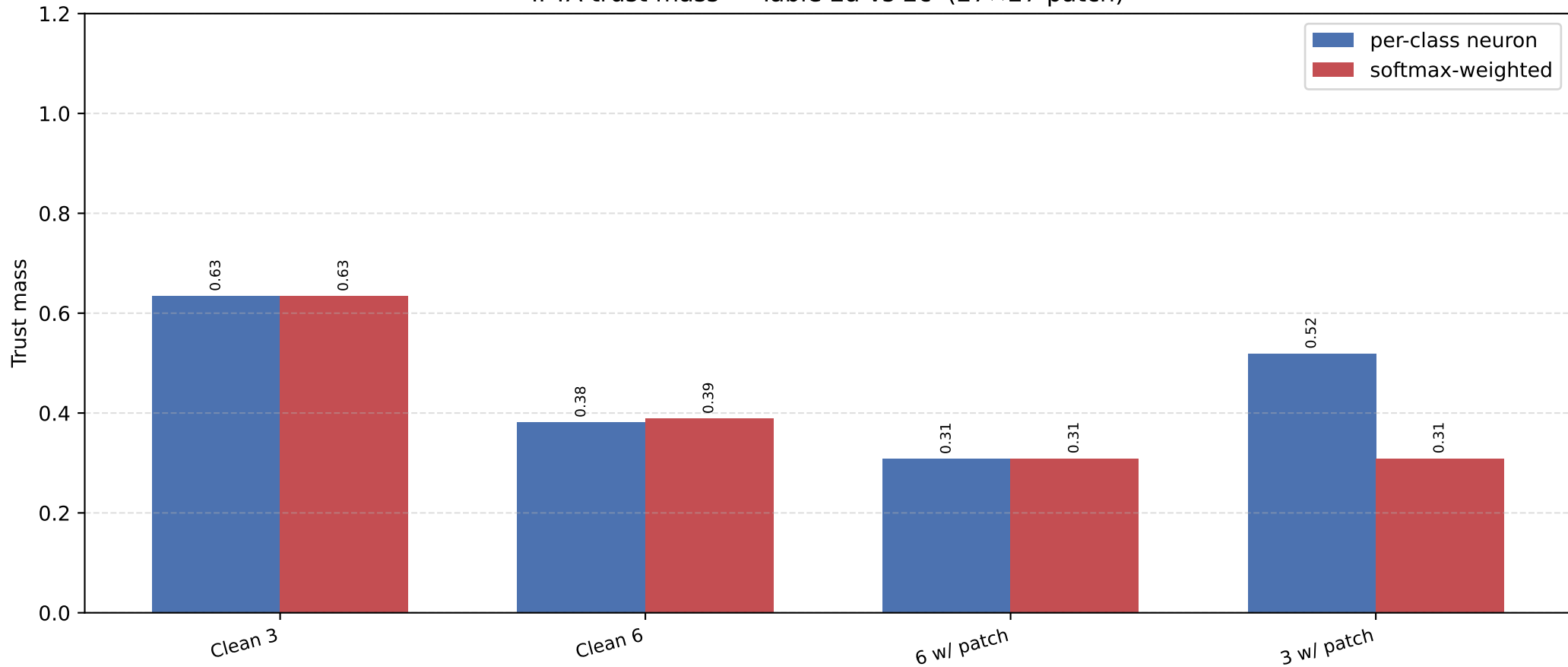
IPTA trust mass — Table 2a vs 2c (27×27 patch)
