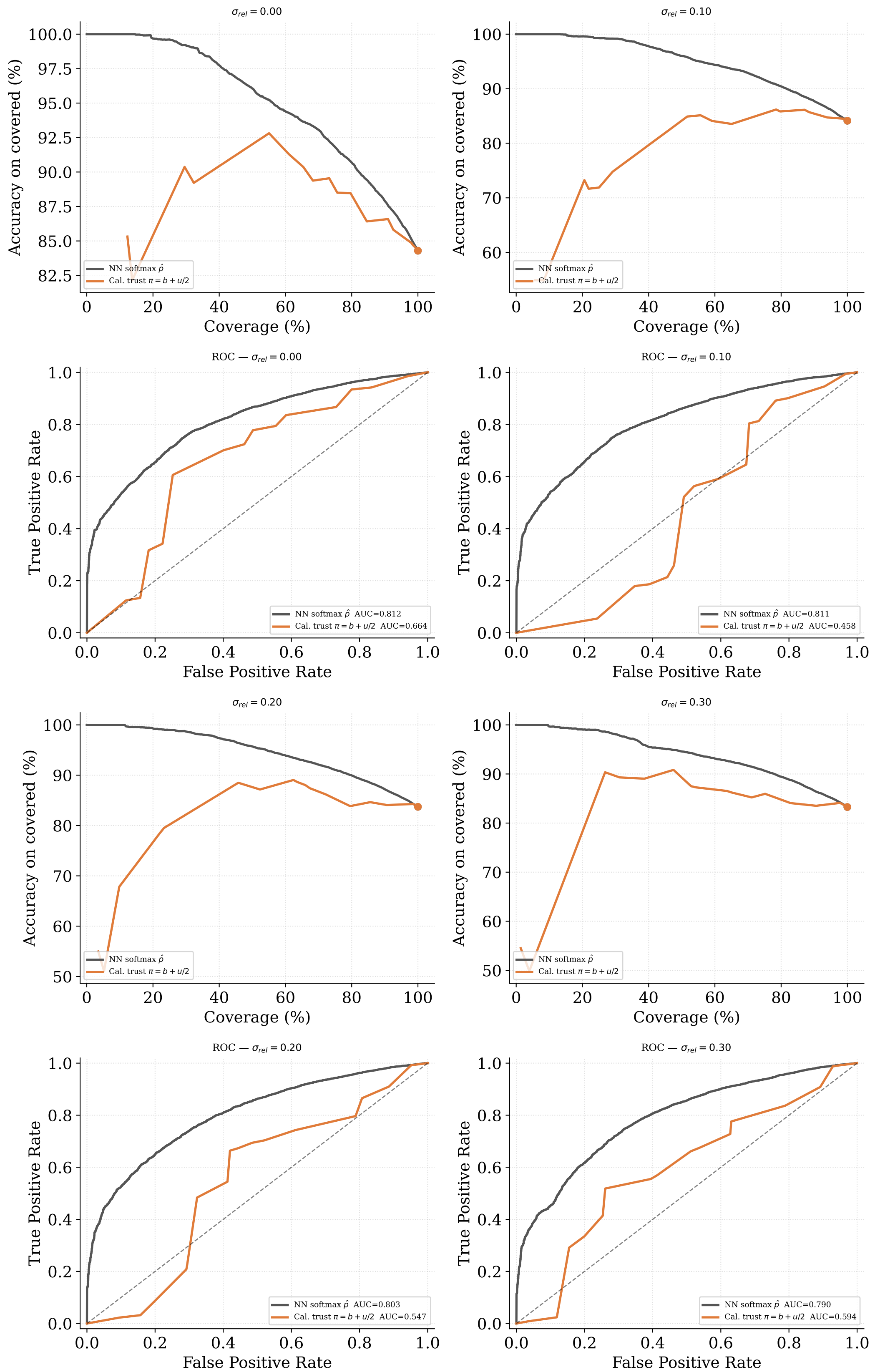
Calibration-based Coverage-Accuracy & ROC — Feature noise ( \pi = b + u/2 threshold vs.\ NN softmax)
