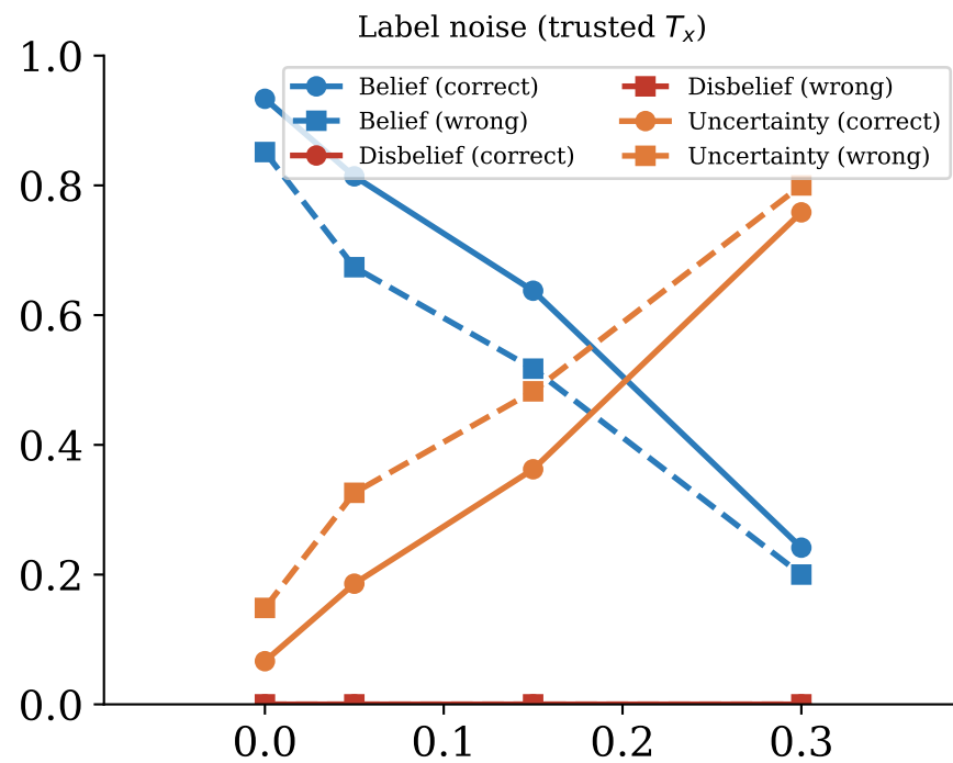
PaTAS confidence signal: opinion masses in predicted class
