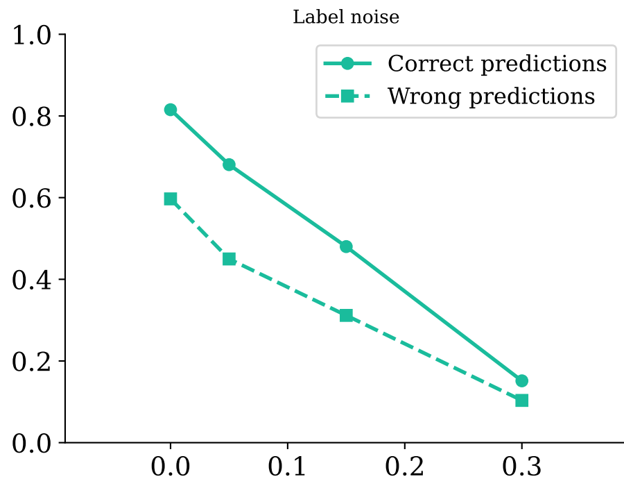
PaTAS signal: correct vs. wrong predictions
