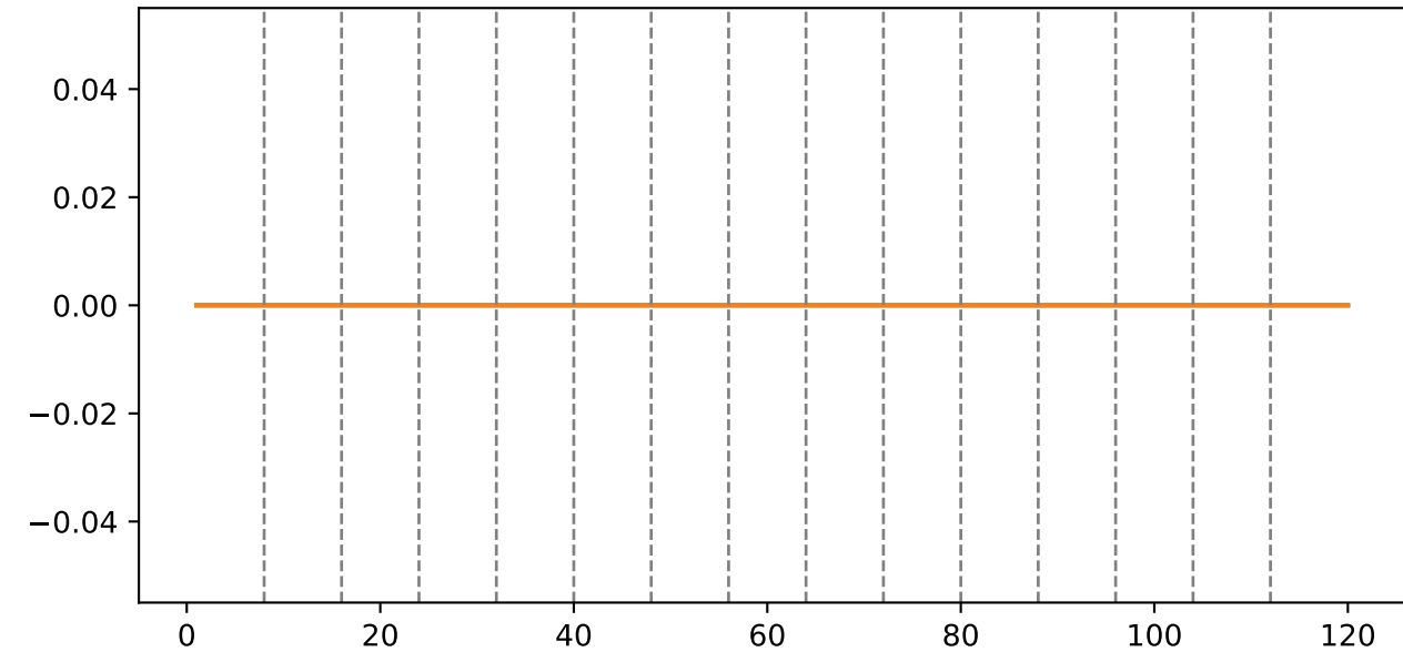
Evolution of distrust mass for vacuous input
