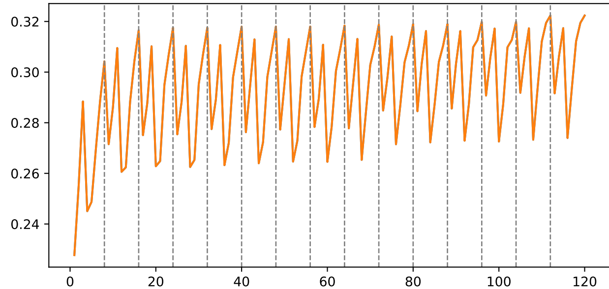
Evolution of trust mass for vacuous input
