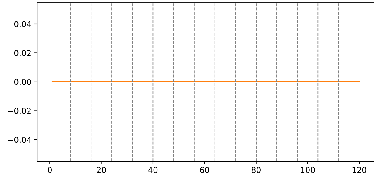
Evolution of distrust mass for fully distrusted input
