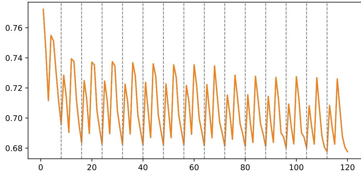
Evolution of uncertainty mass for fully distrusted input
