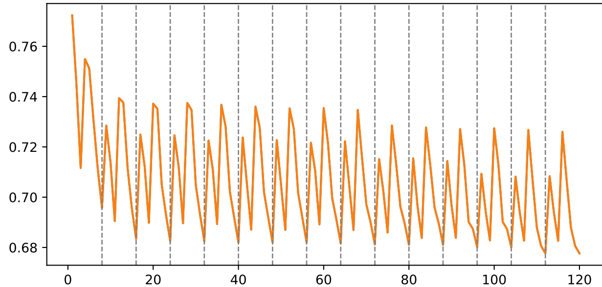
Evolution of uncertainty mass for vacuous input
