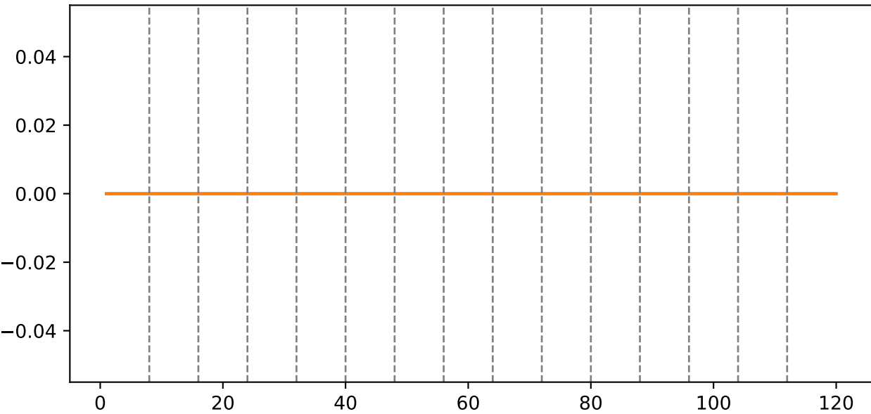
Evolution of trust mass for fully distrusted input
