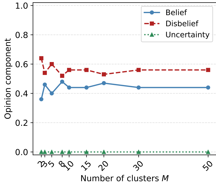
DEMO — Trust opinion vs. number of clusters (epoch 30) Before Calibration After Calibration
