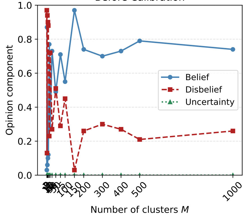
MNIST — Trust opinion vs. number of clusters (epoch 100) Before Calibration After Calibration
