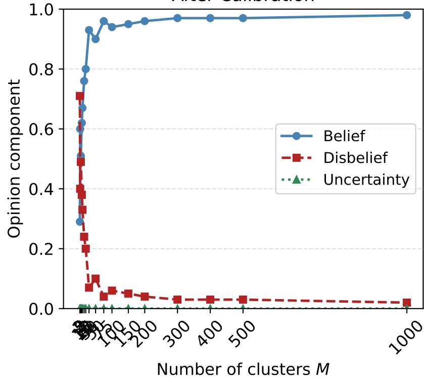
MNIST — Trust opinion vs. number of clusters (epoch 100) Before Calibration After Calibration
