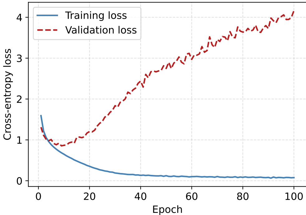
CIFAR — Training and Validation Loss
