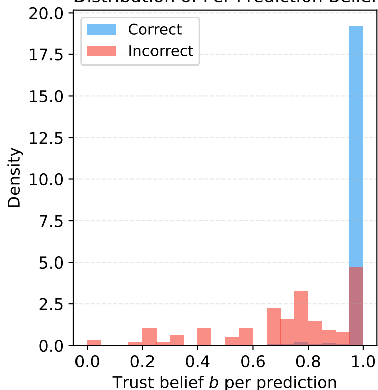
Distribution of Per-Prediction Belief
