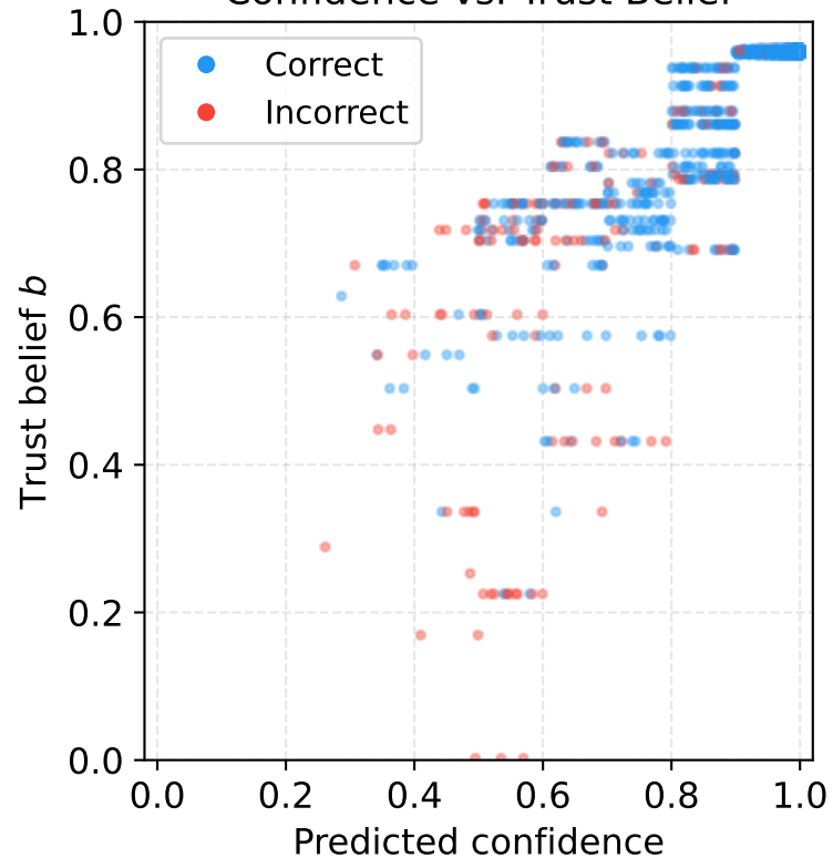
Confidence vs. Trust Belief
