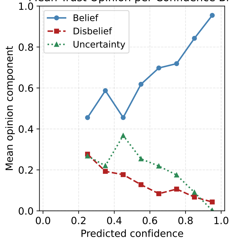
Mean Trust Opinion per Confidence Bin
