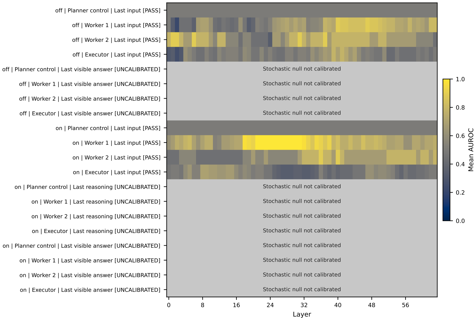
Checkpoint-qualified AUROC across all layers (n=9 domains)
