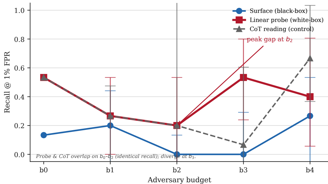
A. Detection recall across the budget ladder
