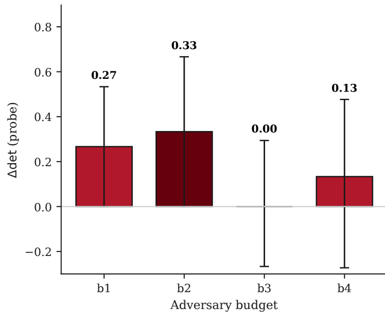
B. Probe robustness gap \Delta\text{det}(b)
