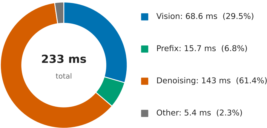
MacBook Pro (Apple M5 Pro, 16-core GPU)
