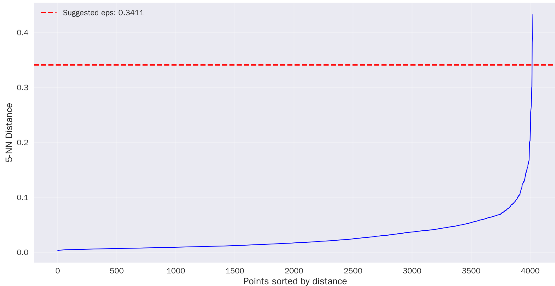
K-Distance Graph (k=5) for Epsilon Estimation
