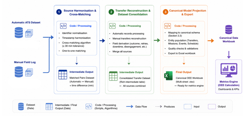
Figure 3.1: End-to-end processing pipeline for canonical-model ingestion
