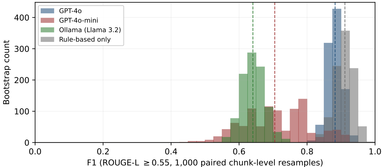
Bootstrap F1 distribution per method (paired resamples, B = 1,000)
