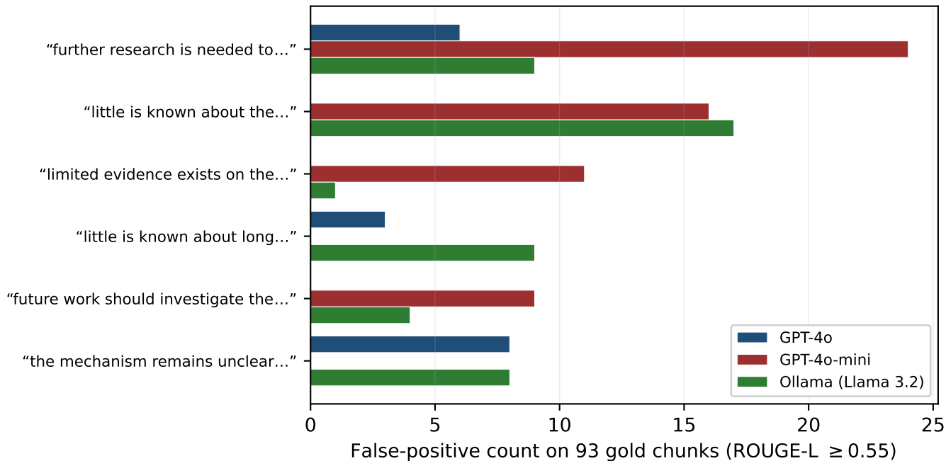
Top false-positive cue patterns per model
