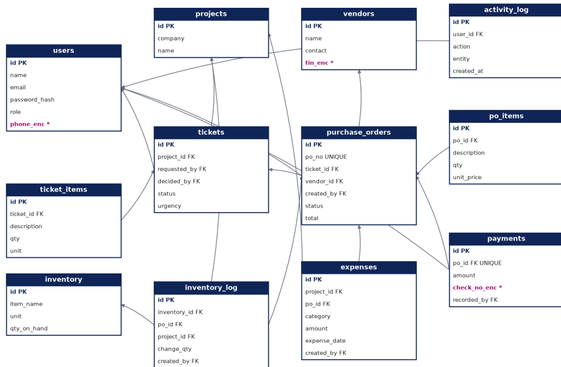
Figure 1. Entity relationship diagram of the rsci_sql database.
