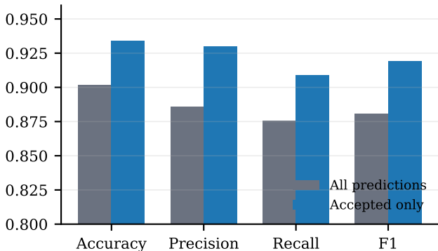
Selective prediction at 90.40% coverage
