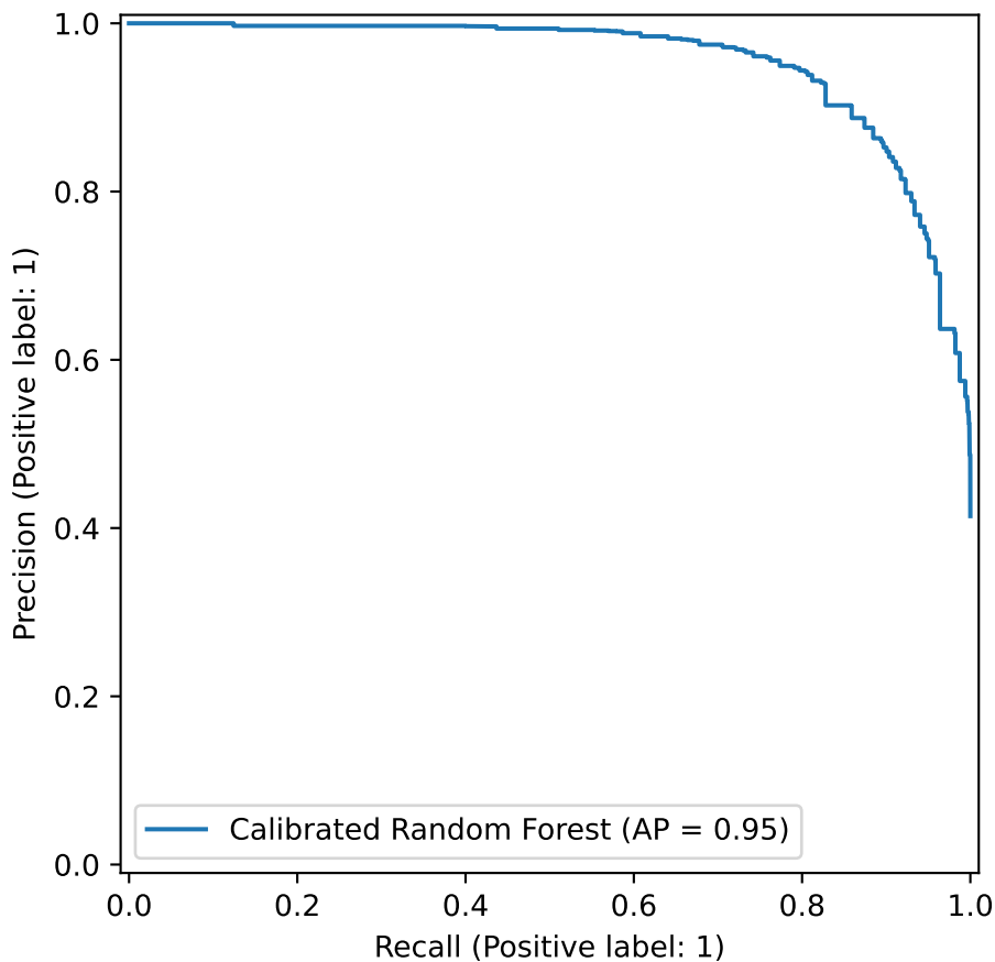
Precision-recall curve
