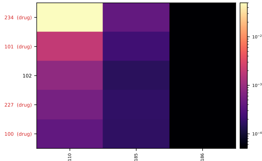
top-5 predicted x active-site (4/5 in drug pocket)
