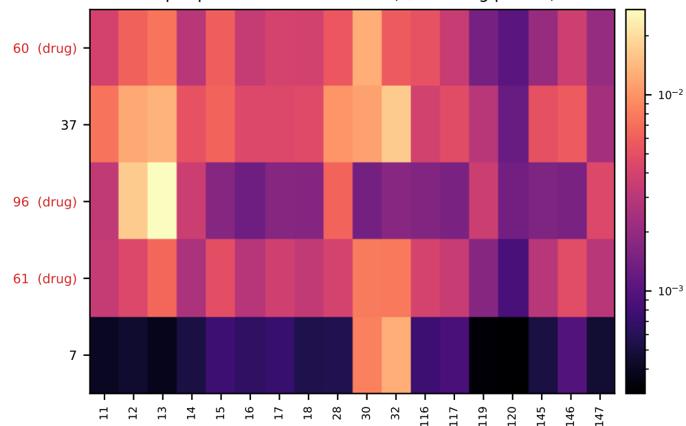
top-5 predicted x active-site (3/5 in drug pocket)
