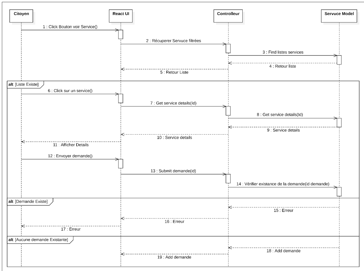
Figure 21 — DS-07 : Consultation des services offerts (BF7)
