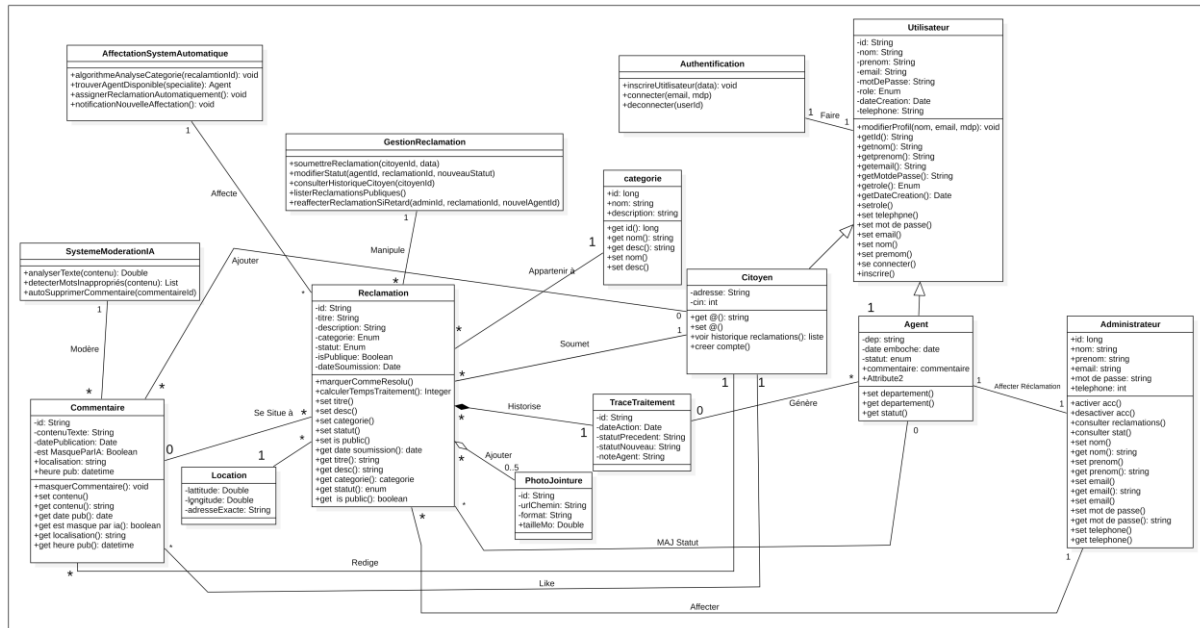
Figure 3 — Diagramme de Classes Sprint 1
