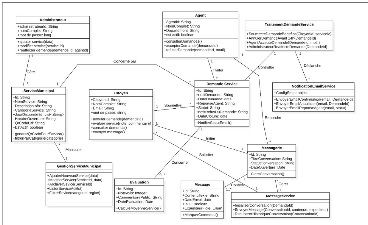
Figure 19 — Diagramme de Classes Sprint 2
