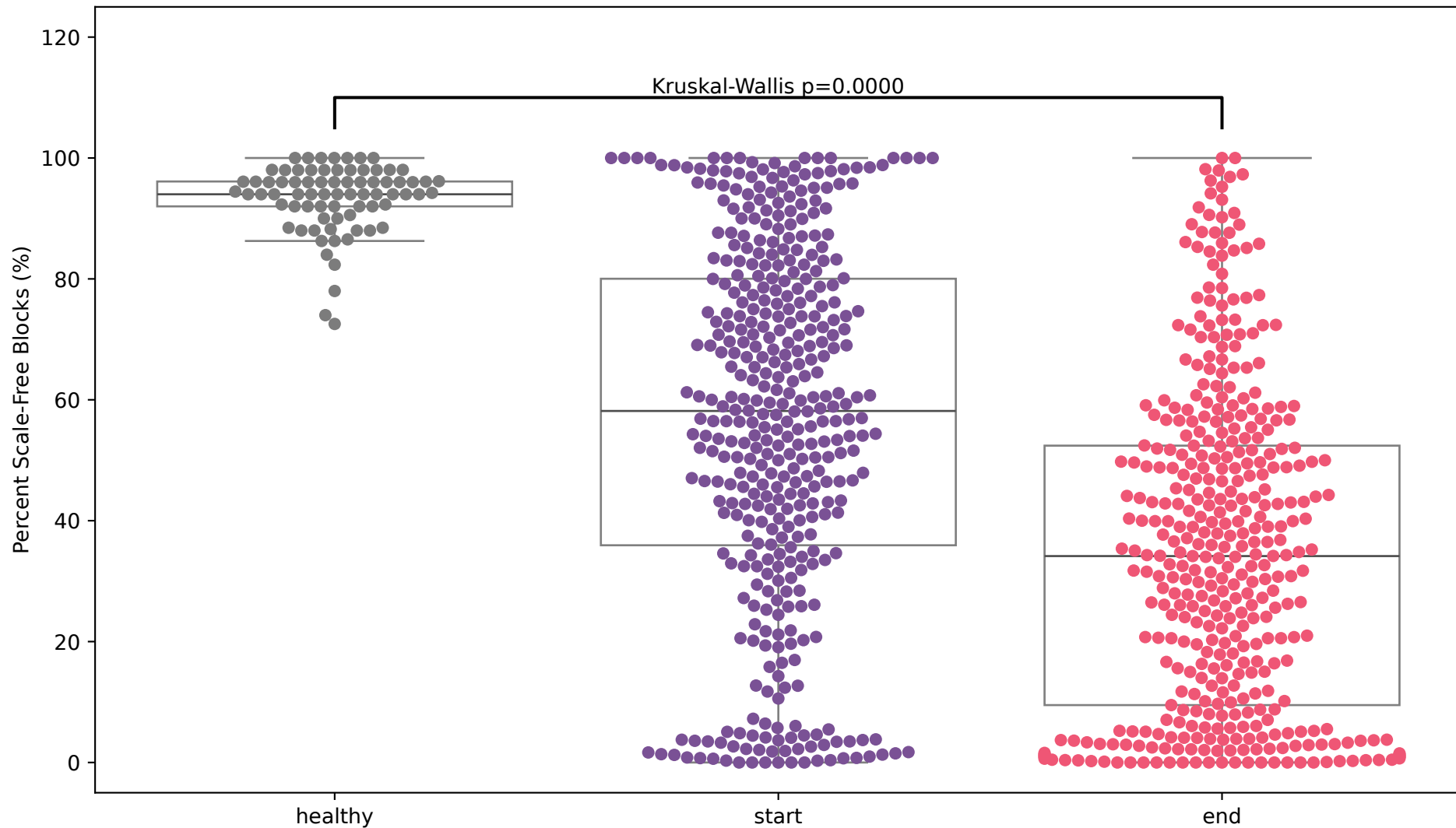
Percent of Blocks Obeying Power Laws per Subject
