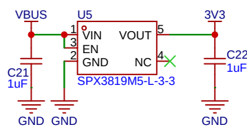
LDO (5V->3V3)
