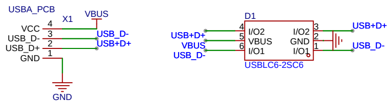
USB + ESD protection
