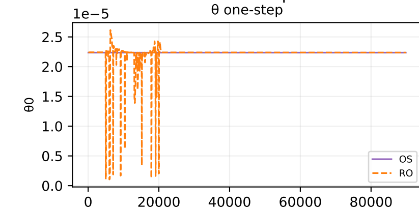
Oracle theta fit — sample 14
