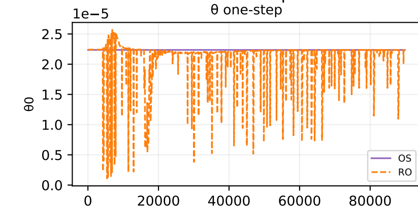
Oracle theta fit — sample 80
