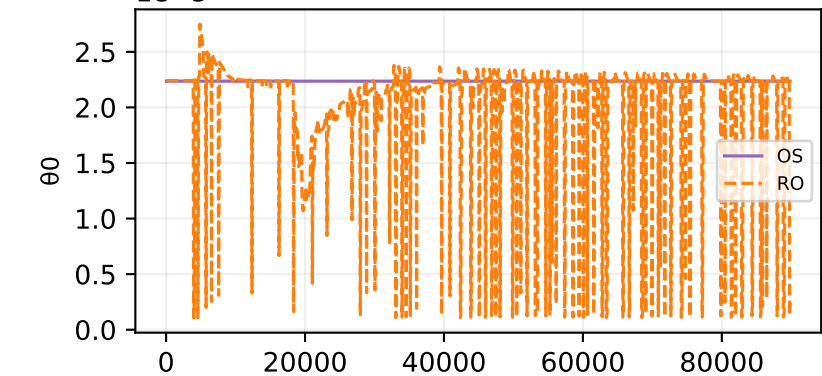
Oracle theta fit — sample 82
