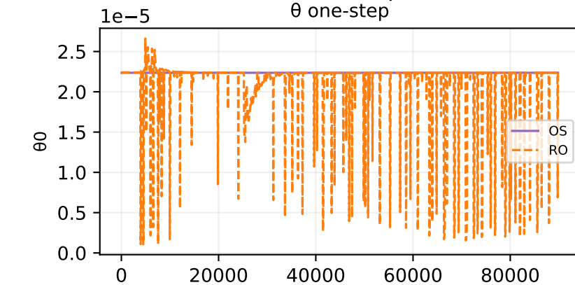
Oracle theta fit — sample 84
