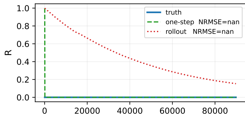
Predictions
