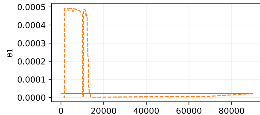
\theta rollout
