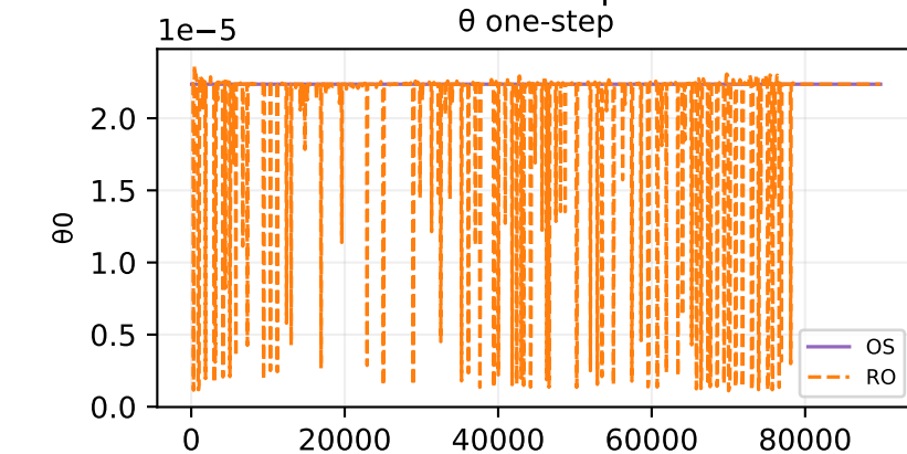
Oracle theta fit — sample 160
