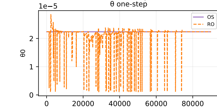
Oracle theta fit — sample 193
