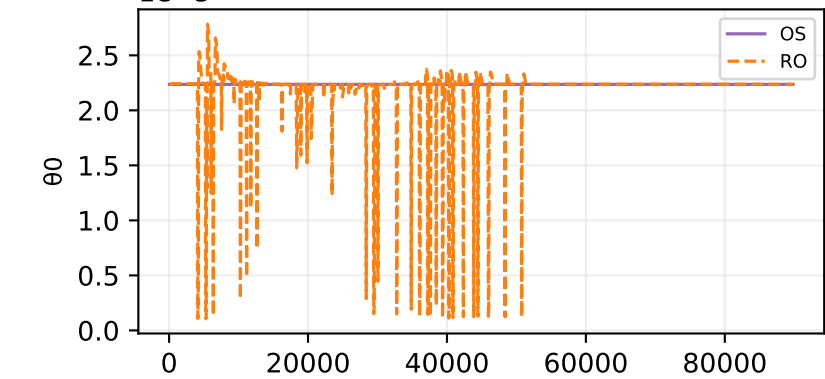
Oracle theta fit — sample 235
