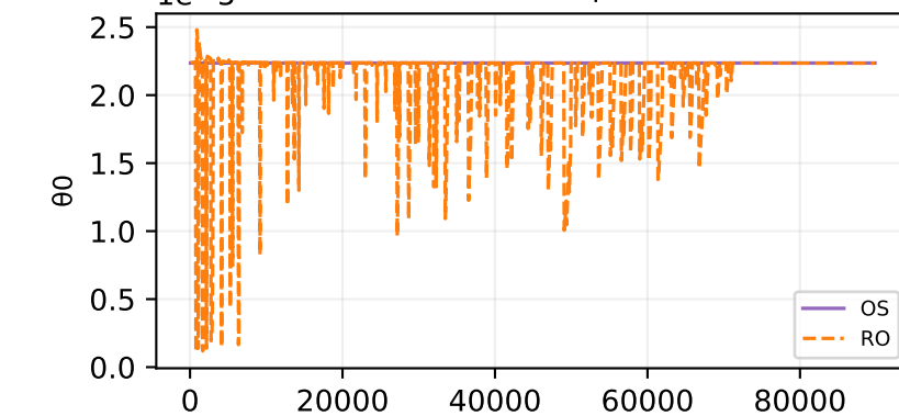
Oracle theta fit — sample 262
