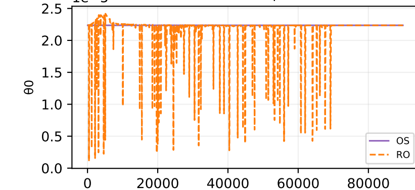
Oracle theta fit — sample 358 \theta one-step
