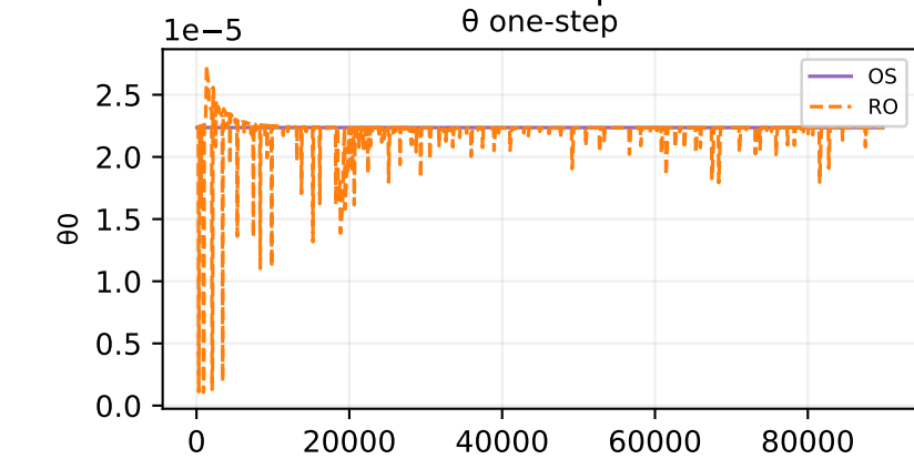
Oracle theta fit — sample 385
