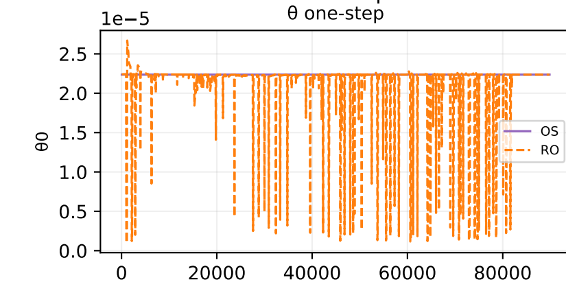
Oracle theta fit — sample 416
