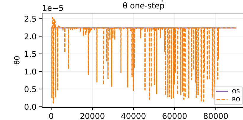
Oracle theta fit — sample 430
