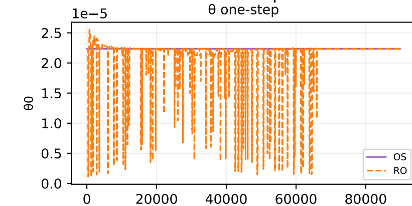
Oracle theta fit — sample 533 \theta one-step
