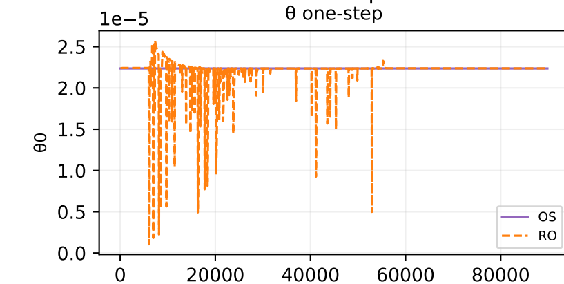
Oracle theta fit — sample 652
