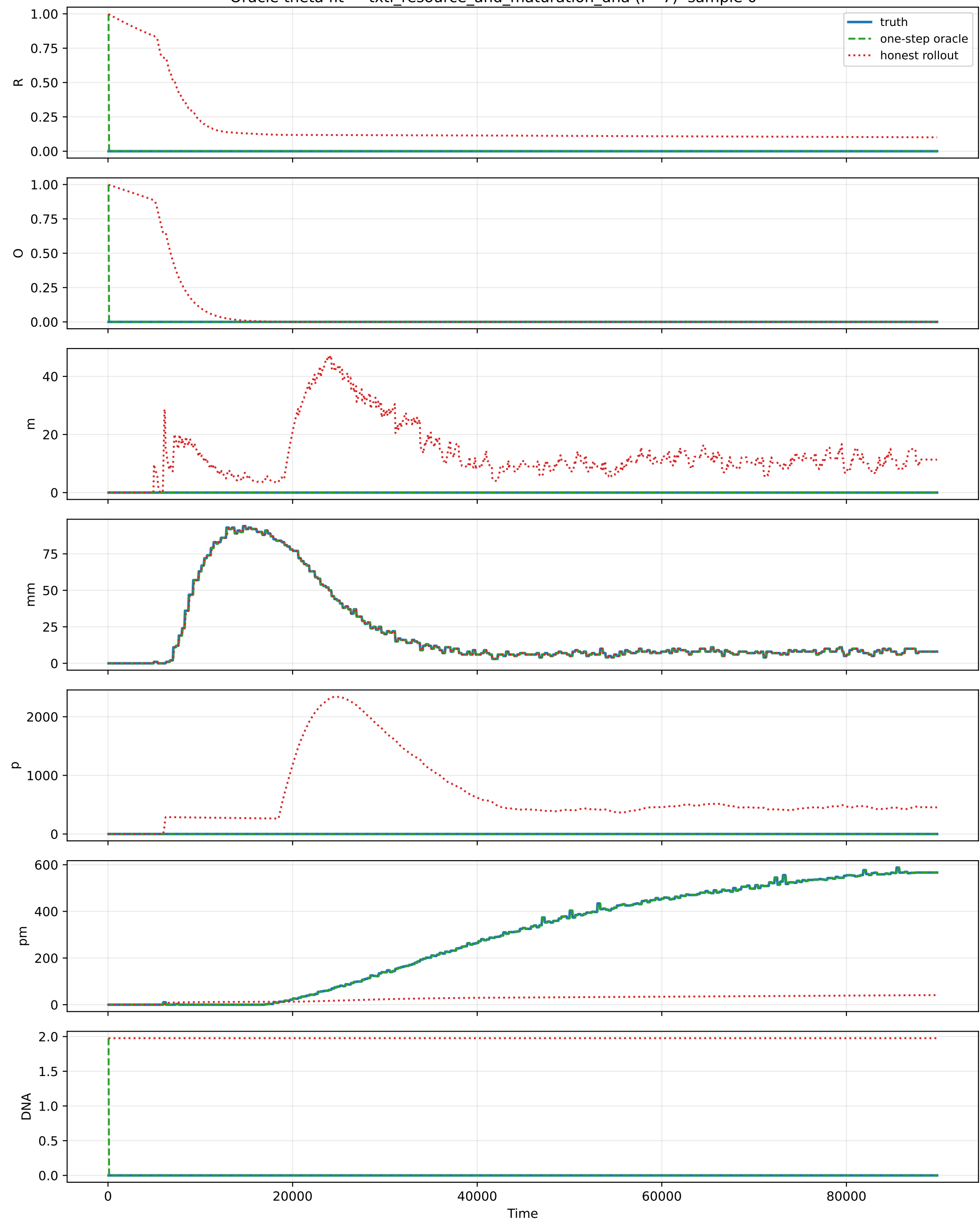
Oracle theta fit — txtl_resource_and_maturation_dna (P=7) sample 0
