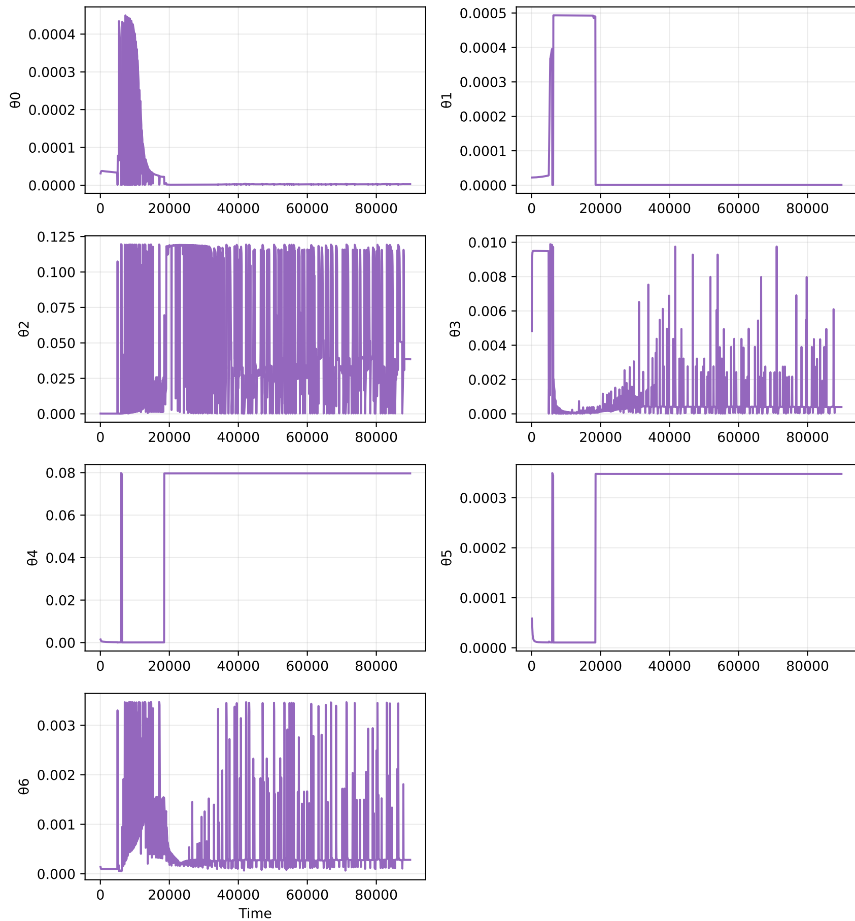
Oracle theta trajectories (rollout) — txtl_resource_and_maturation_dna (P=7) sample 0
