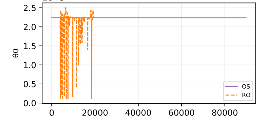
Oracle theta fit — sample 63 \theta one-step
