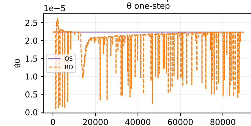
Oracle theta fit — sample 120
