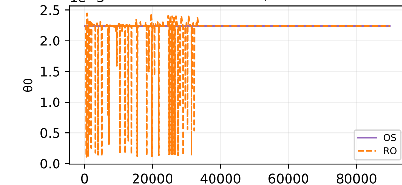
Oracle theta fit — sample 183
