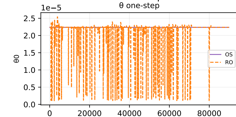
Oracle theta fit — sample 333
