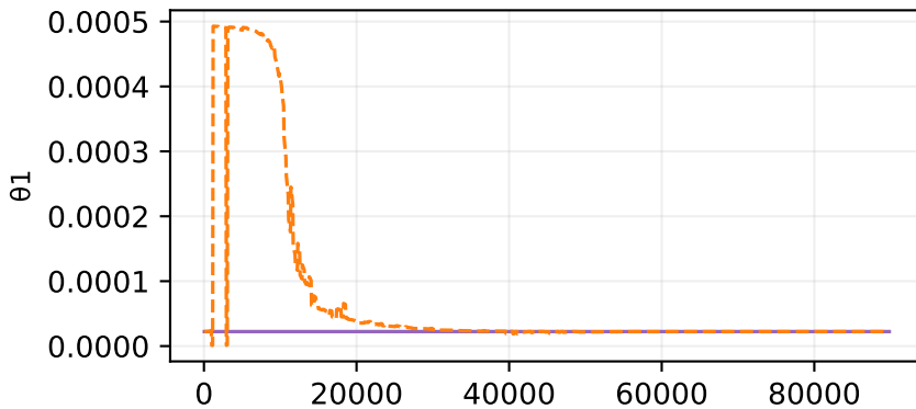
\theta rollout
