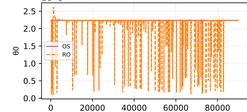
Oracle theta fit — sample 418
