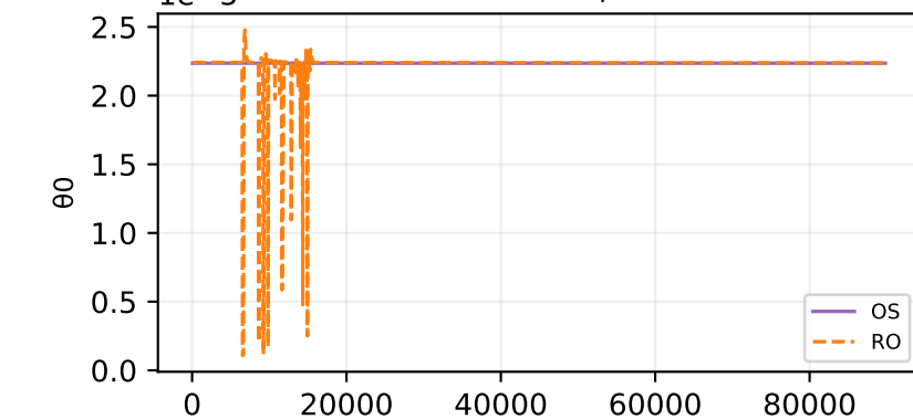
Oracle theta fit — sample 560 \theta one-step
