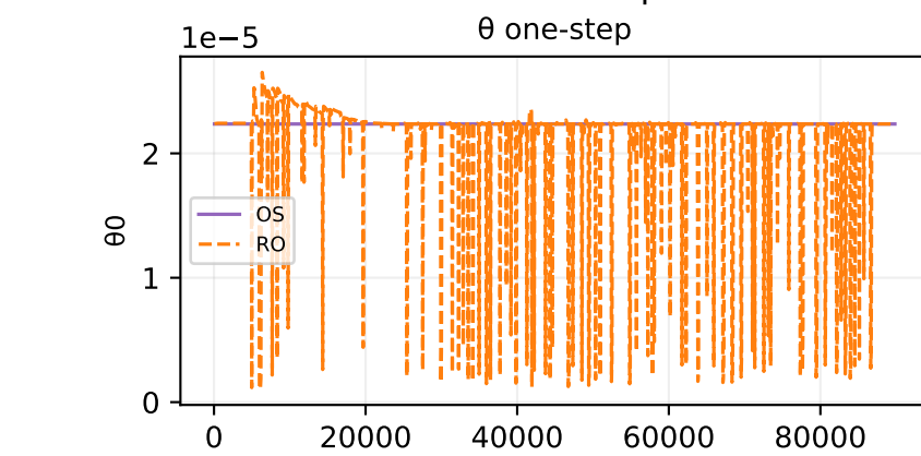
Oracle theta fit — sample 4
