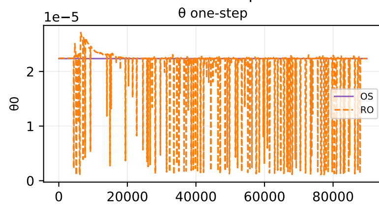
Oracle theta fit — sample 19
