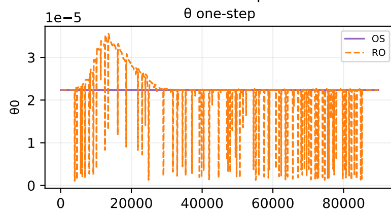
Oracle theta fit — sample 24
